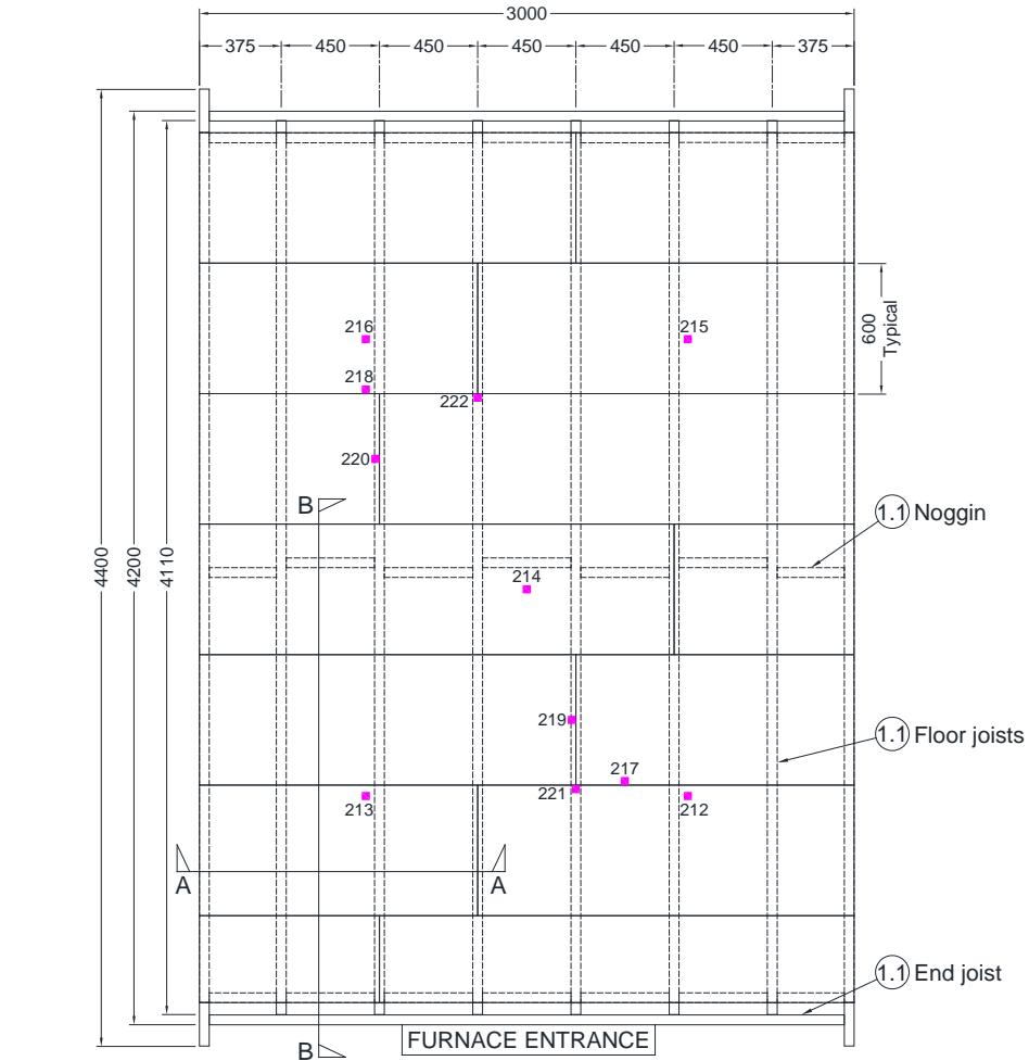
Key ■ Surface thermocouple PLAN OF THERMOCOUPLE POSITIONS
